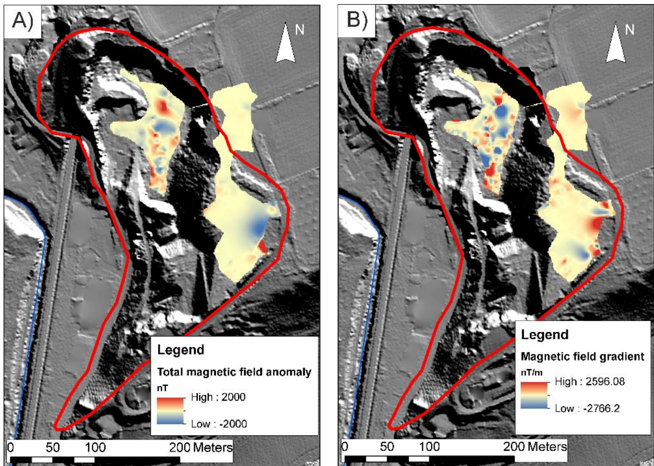
Figure 4: Results of MAG surveys with total magnetic field measured (A) and magnetic field gradient (B). The large anomalies observed in Zone II are attributed to buried magnetic objects (rebars, car parts, etc.).
