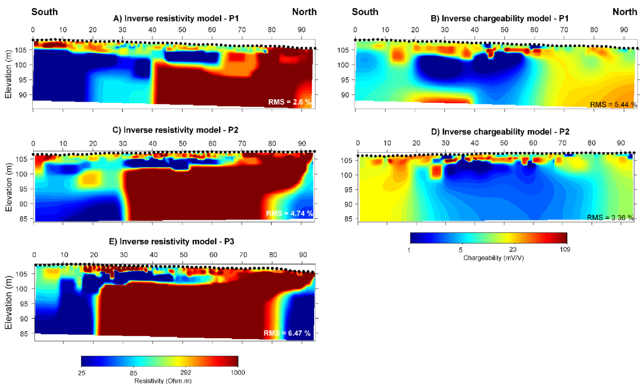
Figure 5: Resistivity (A, C, E) and chargeability (B, D) models obtained inversion of data collected in P1 (A, B), P2 (C, D) and P3 (E). The limestone bedrock is characterized by very high electrical resistivity. Very low resistivity zones are interpreted as ash/lime. Waste close to the soil surface are rather characterized by more heterogeneous electrical properties.
