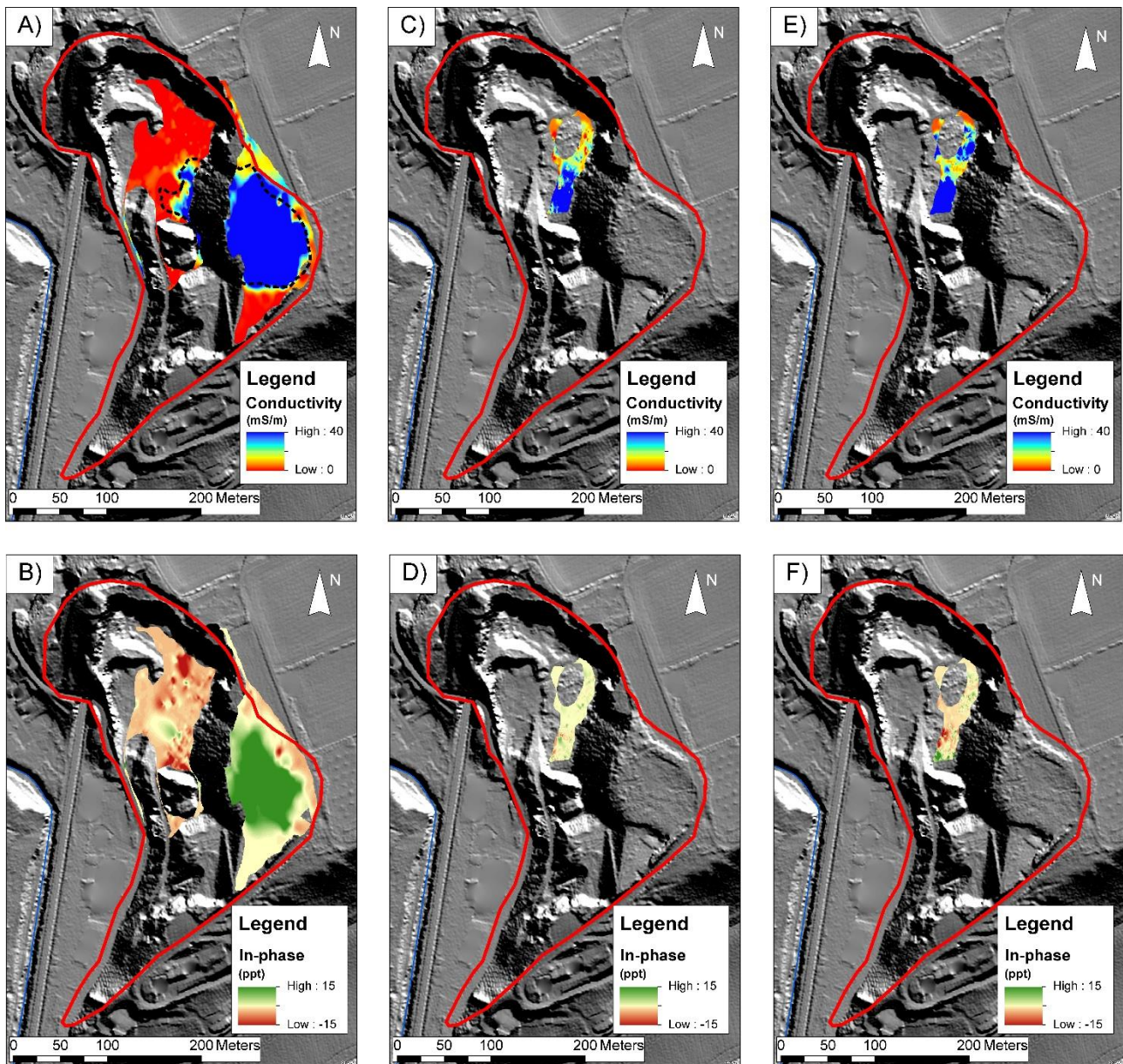
Figure 3: Results of EM surveys with electrical conductivity maps (A, C, E) derived from the quadrature-phase data and in-phase maps related to magnetic susceptibility (B, D, F) at a sounding depth of 6 m (A, B), 2.5 m (C, D) and 0.5 m (E, F). Maps A and B allow to delineate the lateral extent of ash/lime which fits very well with the contour drawn from the aerial view of 1976 (see Fig. 2C).
