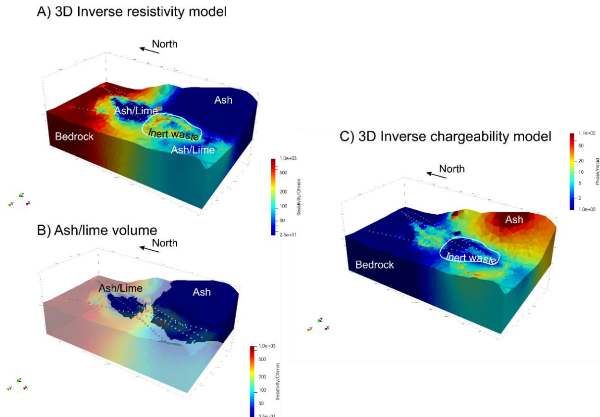
Figure 6: 3D ERT (A) and IP (C) models of Zone II with a proposition of volume of ash/lime estimation by applying a threshold on electrical resistivity value (B).
